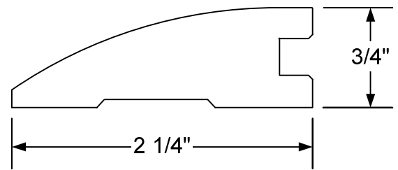
3/4" Reducer
