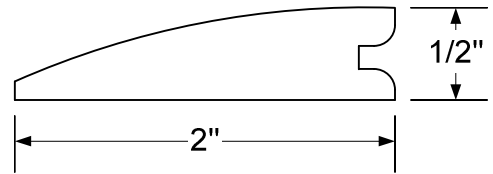
1/2" Reducer
